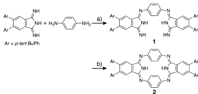
Scheme 1. Synthesis of para -benzihemiporphyrazine 2 . Reaction conditions: a) ethanol, 60 °C, 2 days, b) para -phenylenediamine, 1-chloronaphthalene, 250 °C, 30 min. See Supporting Information (SI) for details. 14
